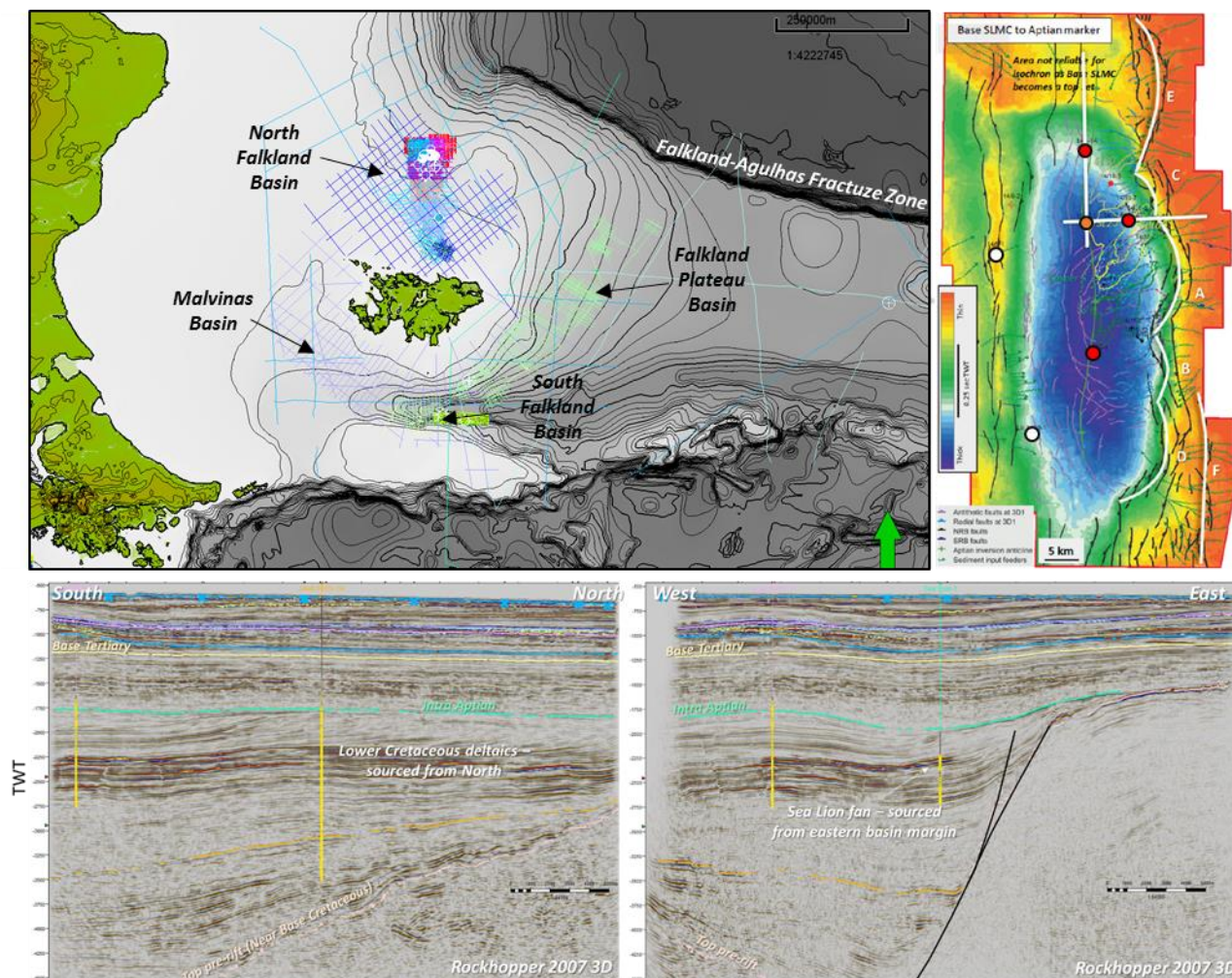
Figure 2. Top Left: Seismic database provided by BGS superimposed on bathymetry map showing the main structural elements of the greater Falkland Plateau and its sub-basins. Additional data will be made available at the end of 2018. Top right shows a Lower Cretaceous isopach map in the North Falklands Basin and location of seismic sections (Lohr and Underhill, 2015). Bottom: TWT seismic sections across the northern North Falkland Basin, showing a range of sediment routing systems supplying sands to the Early Cretaceous lacustrine basin, with turbidites fed by a large southerly-prograding delta system interfingering with point-sourced fan systems derived from the basin margin, including the Sea Lion fan complex.
